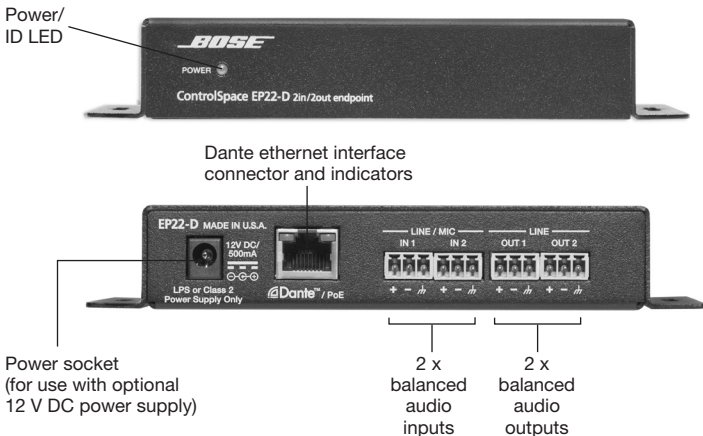
Figure 1. ControlSpace EP22-D 2-in/2-out Dante endpoint front and rear views.
