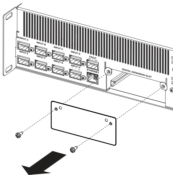
Fig. 1. Remove cover plate from rear expansion slot
