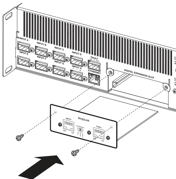
Fig. 2. Insert AmpLink card into amplifier
