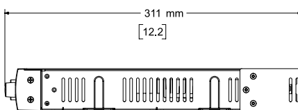
Right View DIMENSIONS APPLY TO BOTH SIDES
