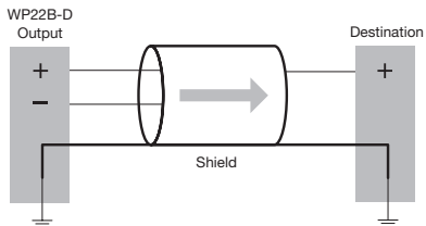
Figure 6. Output to unbalanced destination connection
