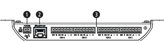
EX-8ML Front View
