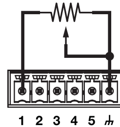
Example: GPI connections for a potentiometer
