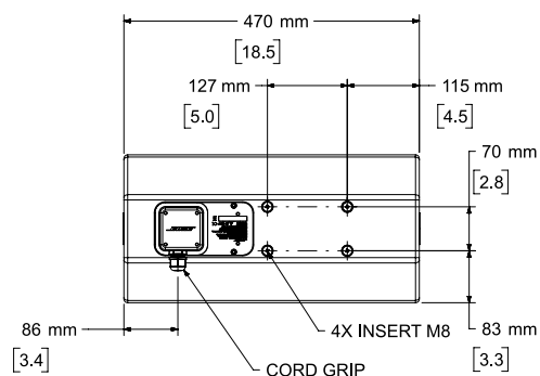
Rear View BRACKET REMOVED FOR CLARITY
