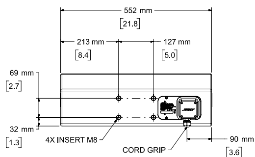
Rear View BRACKET REMOVED FOR CLARITY
