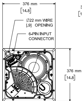
Front View (Grille Removed)
