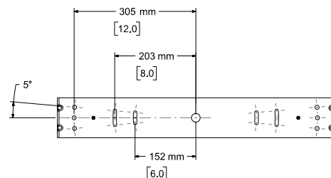
Back View, Bracket
