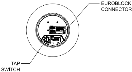
Rear View TOP CAP REMOVED FOR CLARITY
