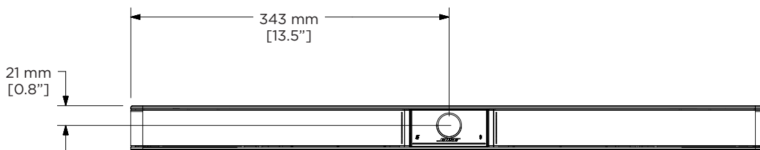
Vista frontal
